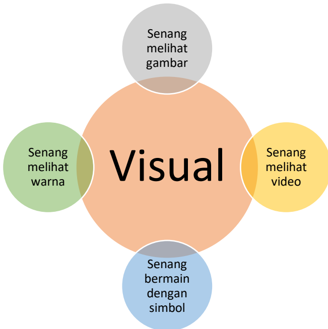
Gambar 1. Model Visual
